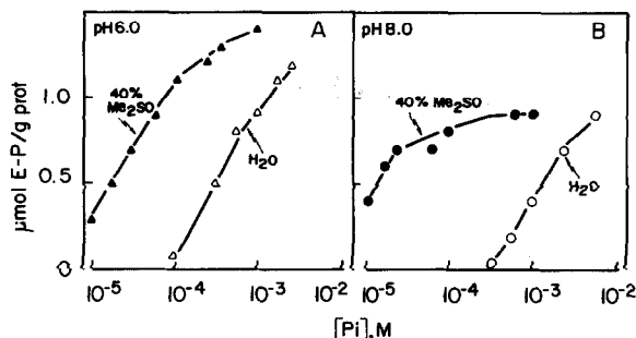
Fig.1. \text{Me}_2\text{SO} and pH effect on \text{P}_i dependence of E-P formation. The assay media contained 10 mM \text{MgCl}_2 , 50 mM Tris-maleate buffer, pH 6.0 (A) or pH 8.0 (B), and the concentration of ^{32}\text{P}_i shown on the abscissa, either without ( \Delta , \circ ) or with 40% (v/v) \text{Me}_2\text{SO} ( \blacktriangle , \bullet ). The reaction was started by the addition of 1.0 mg enzyme protein per ml, and stopped after 2 min at 36^\circ\text{C} with 1 vol. of a cold 10% trichloroacetic acid solution.
